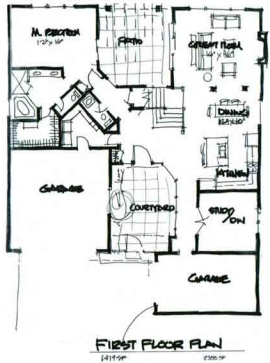
Plan 500 2355 Square Feet
